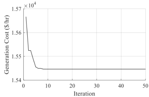
Figure. 4 Convergence graph of PSOHIC
